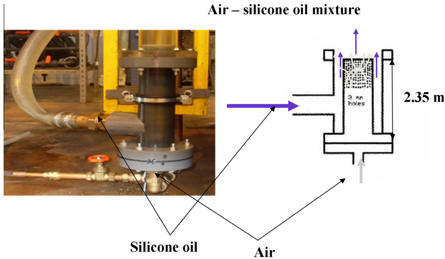
Fig. 1. Air-silicone oil mixing section.
