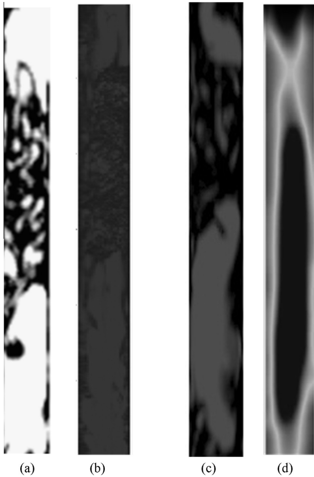
Fig. 6. Comparison of contours of phase distribution at liquid and gas superficial velocities of 0.05 and 0.344 m/s, respectively for between (a) CFD and (b) WMS and for (c) CFD and (d) ECT. For the CFD and WMS comparison, the liquid and gas phases are represented by black and grey colours, respectively. On the contrary, black represents gas phase for the ECT. The initial conditions are riser full of (static) liquid and riser full of air, for CFD and experiment, respectively.
