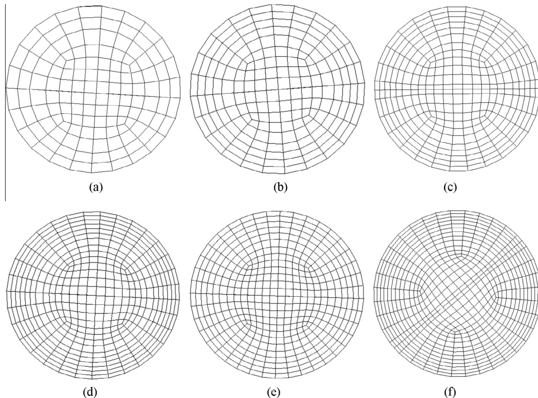
Fig. 4. Cross-sectional view of different sizes of computational grid used for mesh independent study (a) 26,400 cells, (b) 36,000 cells, (c) 54,600 cells, (d) 76,800 cells, (e) 84,000 cells and (f) 102,600 cells. Liquid and gas superficial velocities = 0.05 and 0.344 m/s, respectively. An initial condition of riser full of (static) liquid was used.
