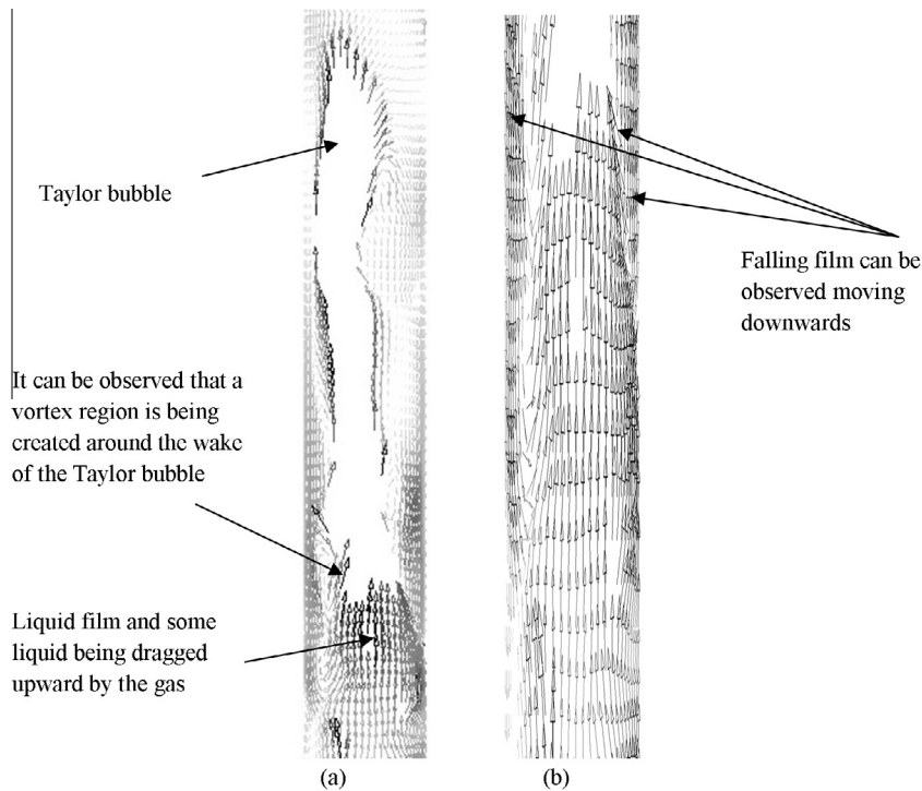
Fig. 8. Velocity field around the (a) Taylor bubble, (b) wake region of the Taylor bubble at liquid and gas superficial velocities of 0.05 and 0.344 m/s, respectively. The initial conditions are riser full of (static) liquid and riser full of air, for CFD and experiment, respectively.
