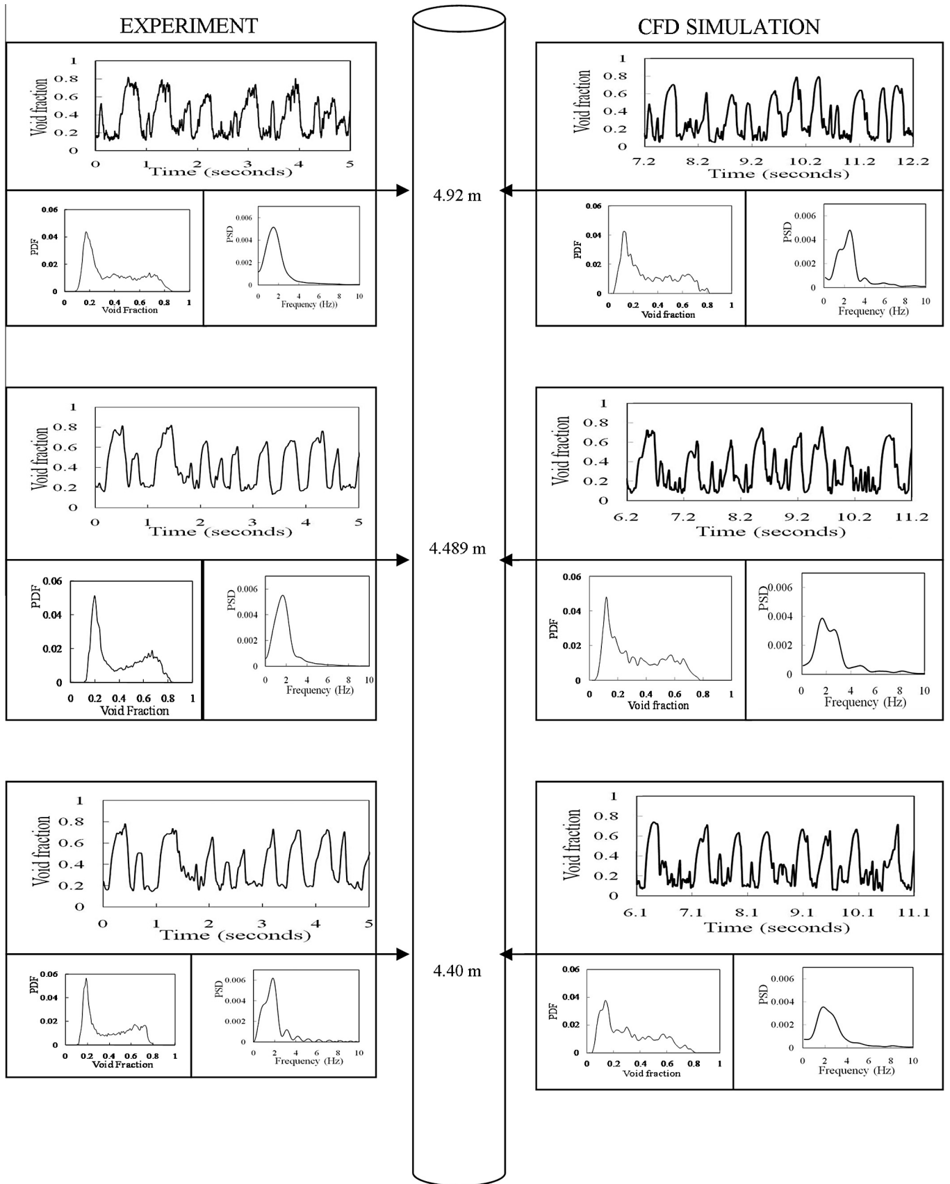
Fig. 5. Comparison between experimental data and CFD simulation results at liquid and gas superficial velocities of 0.05 and 0.344 m/s, respectively. The initial conditions are riser full of (static) liquid and riser full of air, for CFD and experiment, respectively. The time difference observed in the CFD is due to the different times recorded for the Taylor bubble to arrive the measurement locations. Locations 4.4 m, 4.489 m and 4.92 m corresponds to ECT-plane 1, ECT-plane 2 and WMS, respectively.
