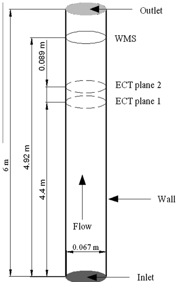
Fig. 2. 3-D geometry of the computational flow domain showing the location of the recording sections that correspond to the locations of the experimental measurement transducers.
