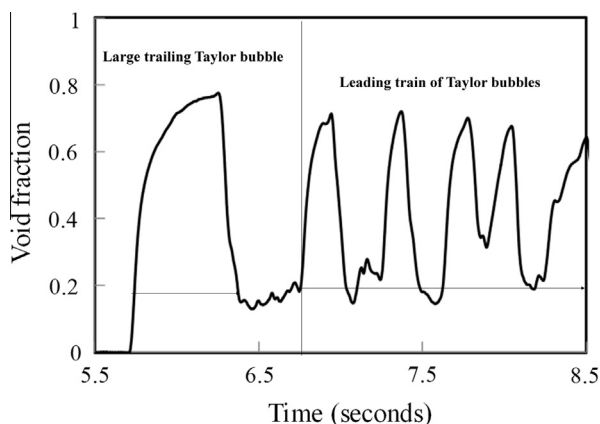
Fig. 9. A plot showing a combination of a large trailing Taylor bubble (start-up) and leading train of smaller Taylor bubbles (steady-state) at liquid and gas superficial velocities = 0.05 and 0.344 m/s, respectively. The initial condition for both CFD and experiment is riser full of (static) liquid.
