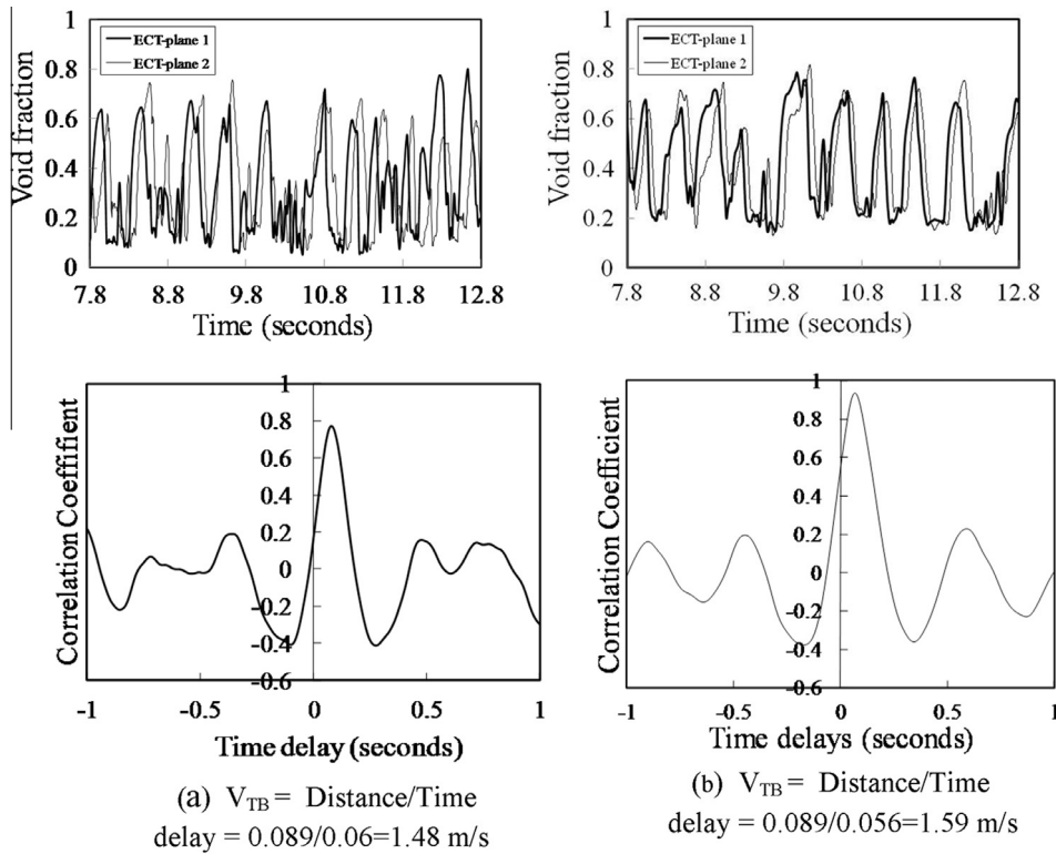
Fig. 10. Time delay of a Taylor bubble passing through two different measuring locations along the pipe. The liquid and gas superficial velocities are 0.05 and 0.344 m/s, respectively (a) CFD and (b) Experiment. The initial condition for both CFD and experiment is riser full of (static) liquid. V_{TB} represents the structure velocity of the Taylor bubble.
