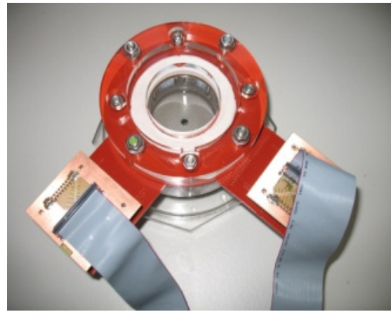
Fig. 2: Wire mesh sensor (WMS)
