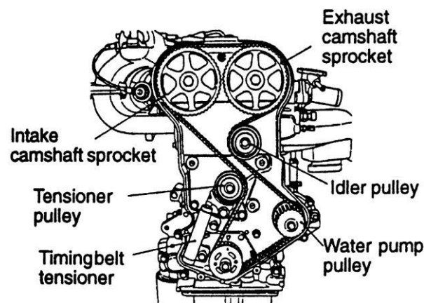
Figure 1: Engine timing system parts identification ( www.autozone.com ).
