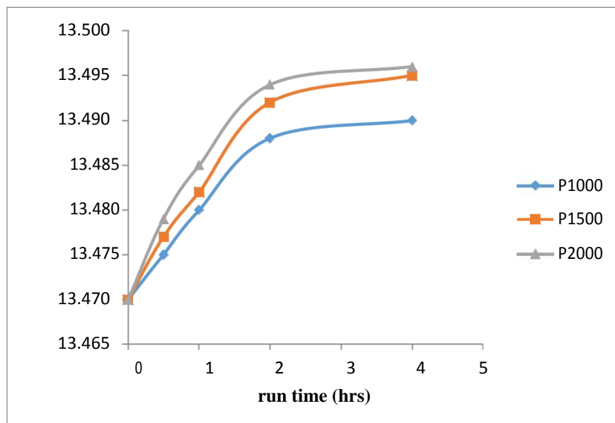
Figure 5: Effect of pitch against run time
