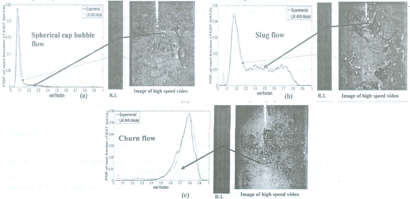
Figure 1: Experimental and predicted PDF of void fraction before the bend at liquid superficial velocity of 0.14 and gas superficial velocity ( \text{ms}^{-1} ) of: (a) 0.05 (b) 0.54 and (c) 2.84 . R.I. represents reconstructed images of two-phase flow pattern. The dash line (a) Represents bubble flow while the thick line spherical cap bubble. On the other hand, the thick line in (b) represents Taylor bubble while the dash line liquid slug. The thick line in (c) represents churn flow.
