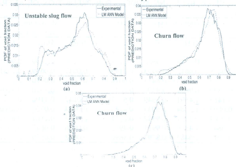
Figure 2: Experimental and predicted PDF of void fraction at liquid superficial velocity of 0.14 and gas superficial velocity ( \text{ms}^{-1} ) of: (a) 0.95 (b) 1.40 and (c) 1.89 .
