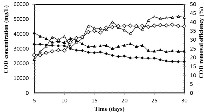
Figure 2. COD concentration and COD percentage reduction of the complete mix anaerobic reactor (▲) R3 COD concentration of pre-treated OPMF + CM; (Δ) R3 COD removal efficiency; (●) R4 COD concentration of untreated OPMF + CM; (○) R4 COD removal efficiency
