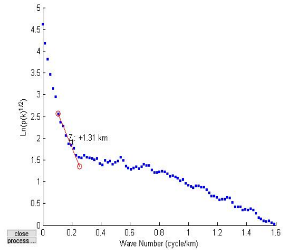
Fig. 5. Z_o and Z_t plots of energy against frequency for block A
