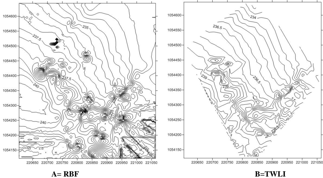
Figure 4: Contour maps generated by Radial Basis Function A), Triangulation with Linear Interpolation B) methods.
