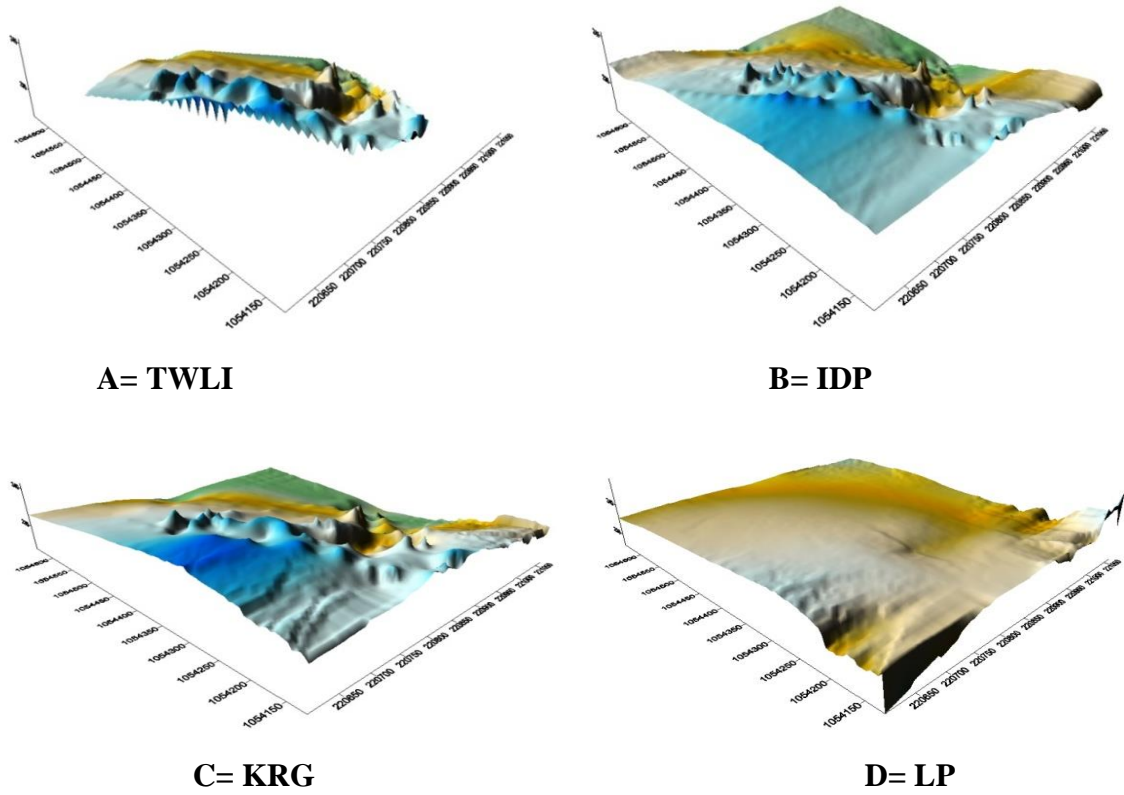
Figure 5: Digital elevation model from triangulation with linear interpolation A), Inverse Distance to Power B), kriging C), and Local Polynomial D) methods.
