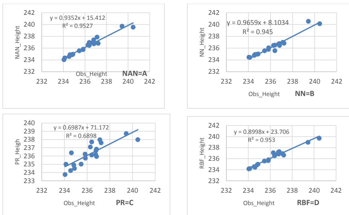
Figure 9: scatter point graph, linear trend line, equation of the curves and R^2 statistics for Natural Neighbor A), Nearest Neighbor B), Polynomial Regression C), and Radial Basis Function D) method.
