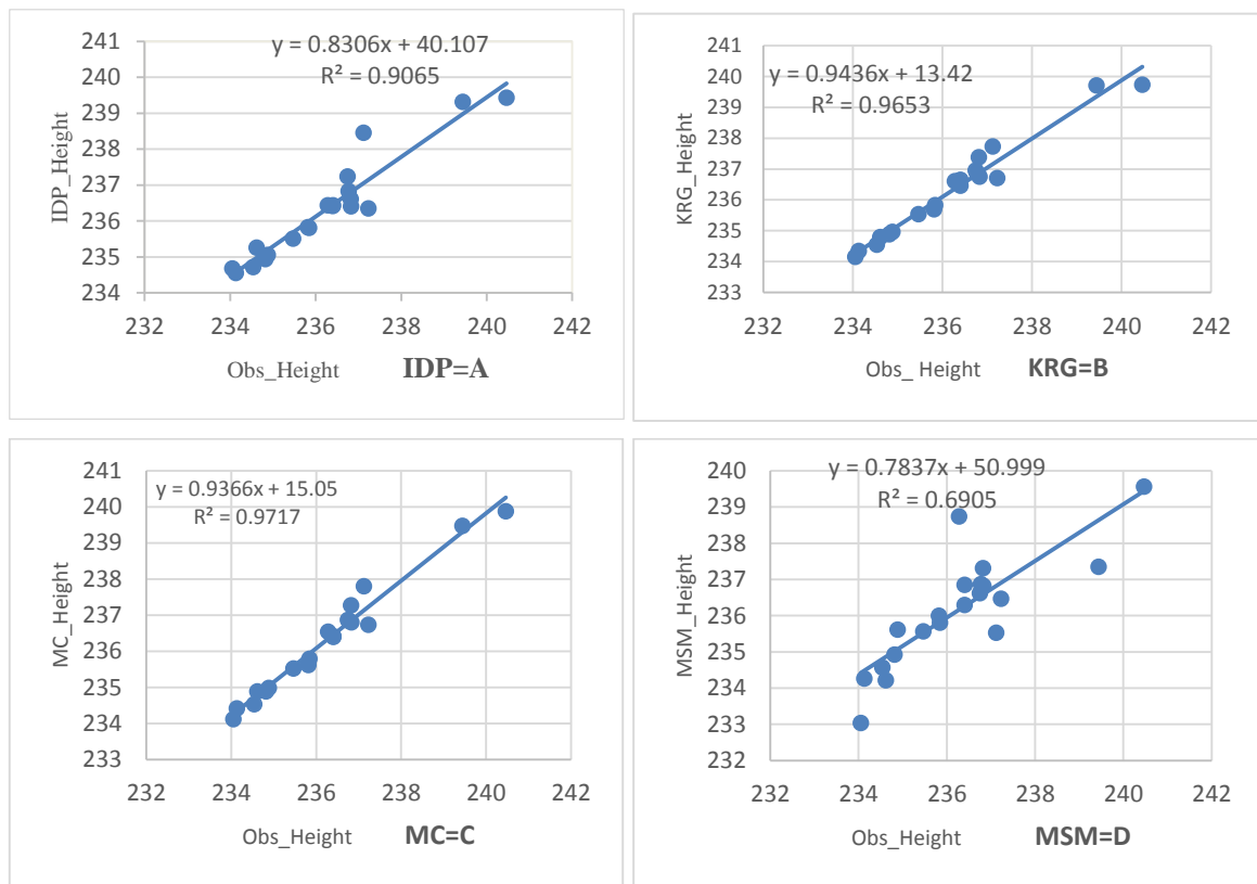
Figure 8: scatter point graph, linear trend line, the equation of the curves and R^2 statistics for Inverse Distance to Power A), Kriging B), Minimum Curvature C), and Modified Shepard method D) methods.
