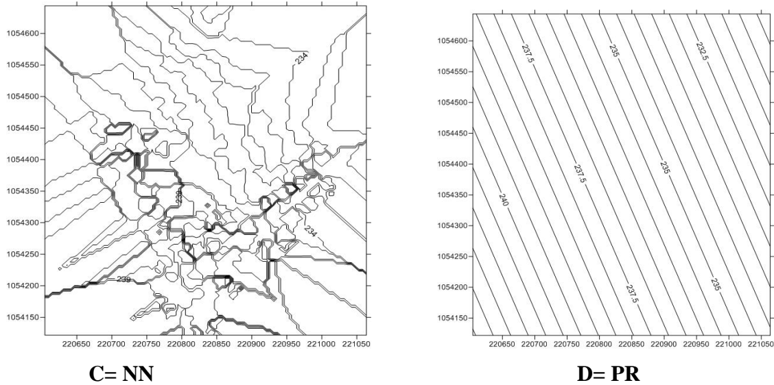
Figure 3: Contour maps generated by Modified Shepard Method A), Natural neighbor B), Nearest neighbor C), Polynomial regression D) methods.
