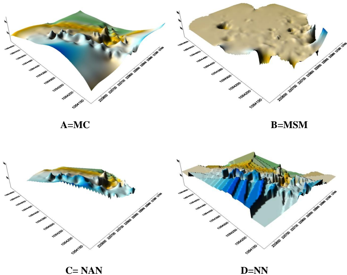
Figure 6: Digital elevation model for Minimum Curvature A), Modified Shepard B), Natural Neighbor C) and Nearest Neighbor D) methods.
