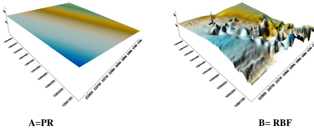
Figure 7: Digital elevation model for Polynomial Regression A), Radial Basis Function B)
