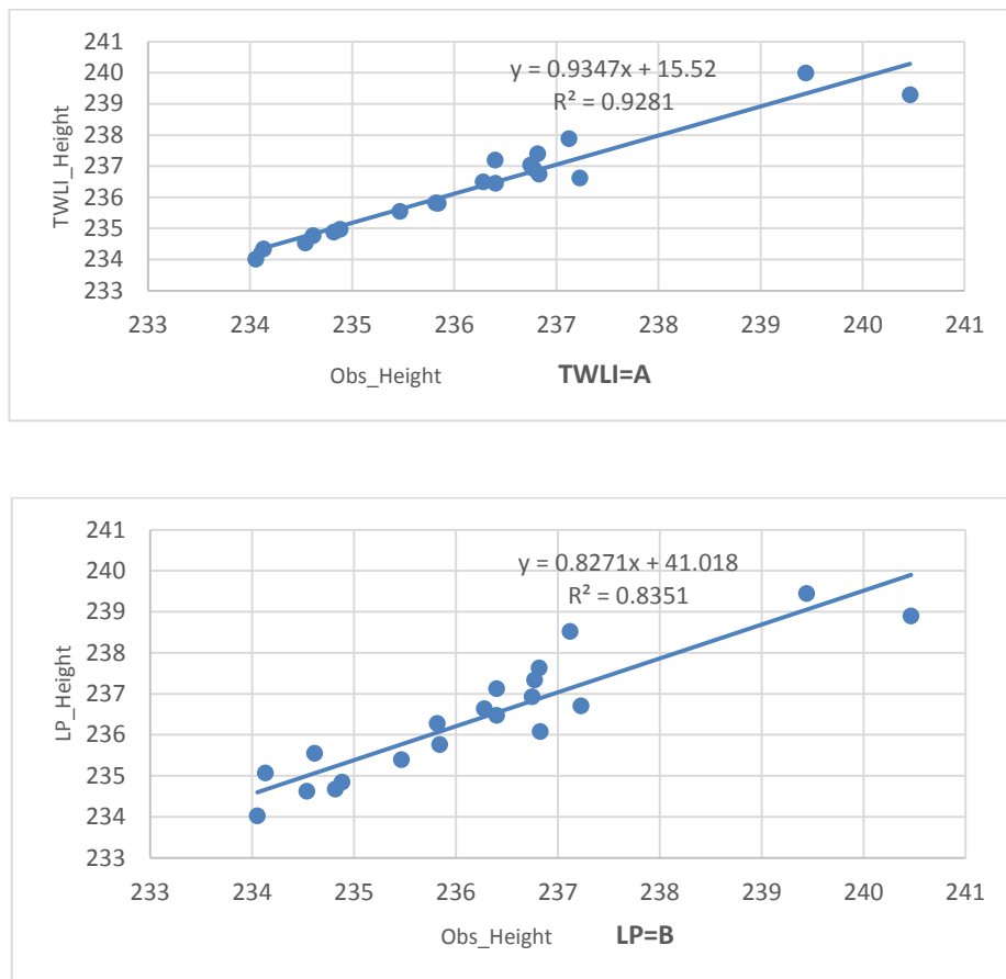
Figure 10: scatter point graph, linear trend line, equation of the curves and R^2 statistics for Triangulation with Linear Interpolation A), Local Polynomial B) method.
