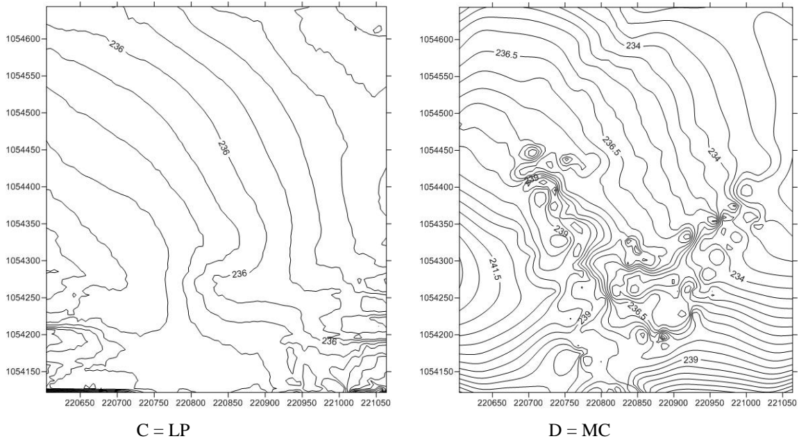
Figure 2: Contour maps generated by Inverse distance to power A), Kriging B), Local polynomial C), and Minimum Curvature D) methods.
