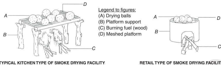
Figure 10.1.3 Typical smoke drying facility for drying fermented cassava mash in West Africa (source: Shittu et al. , 2005).
