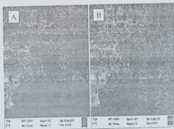
Figure 2 SEM morphology of unmodified (A) and modified (B) kaolinite clay
