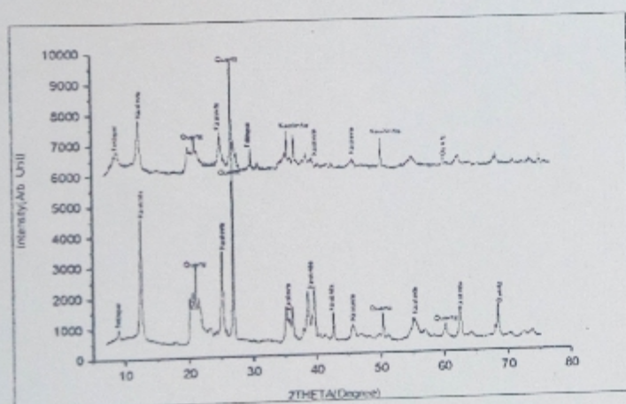
Figure XRD spectra of (A) unmodified and (B) modified kaolinite clay samples
