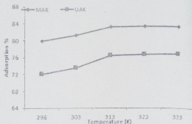
Figure 5 Effect of temperature on Cu (II) ion uptake onto unmodified and modified kaolinite clay
