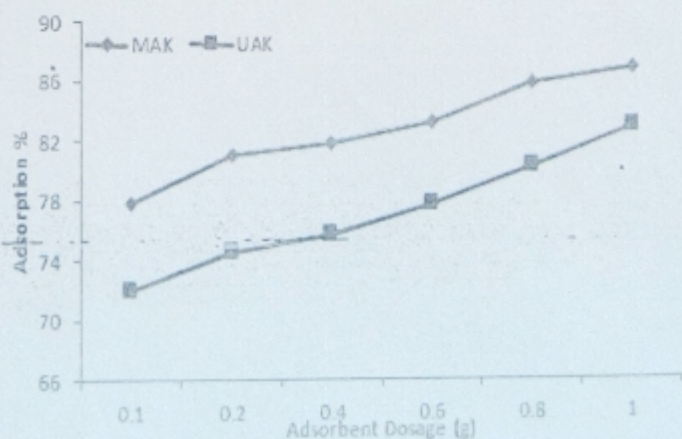
Figure 6 Effect of dosage on Cu (II) ion uptake onto unmodified and modified kaolinite clay
