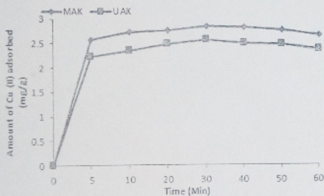
Figure 4 Effect of contact time on adsorption of Cu onto unmodified and modified kaolinite clay
