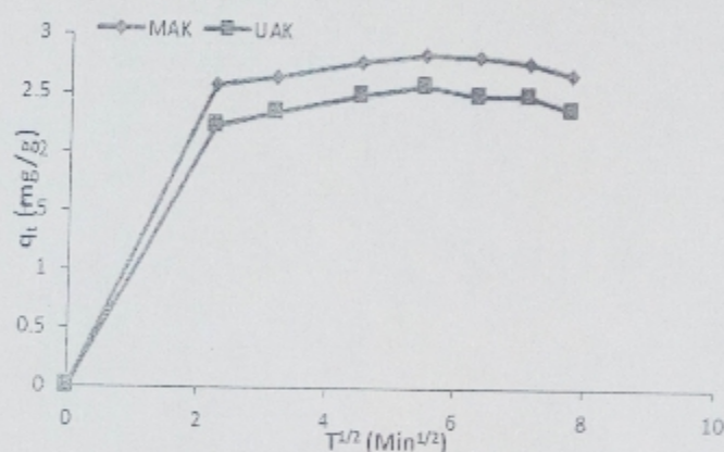
Figure 9 Intra-particle diffusion plot for removal of Cu (II) ion onto unmodified and modified kaolinite
