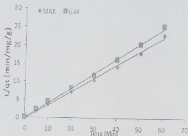
Figure 8 Pseudo second-order kinetic plot for removal of Cu (II) ion onto unmodified and modified kaolinite
